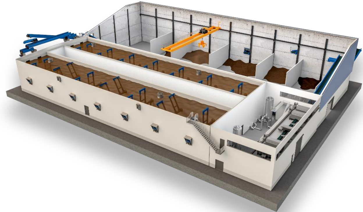
Continuous Fermentation
